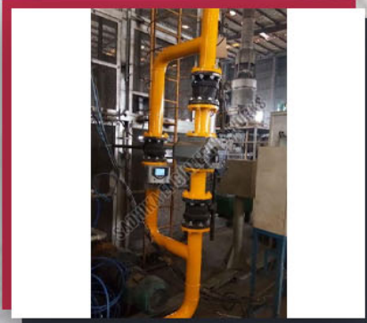
LPG Flow Meter
